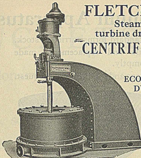
Fletcher Cantilever Suspended Steam Turbine Driven Centrifugal
