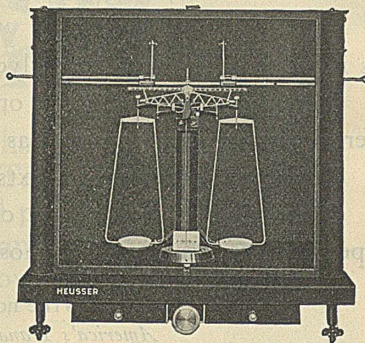
Group "H" Heusser Analytical Balance.
