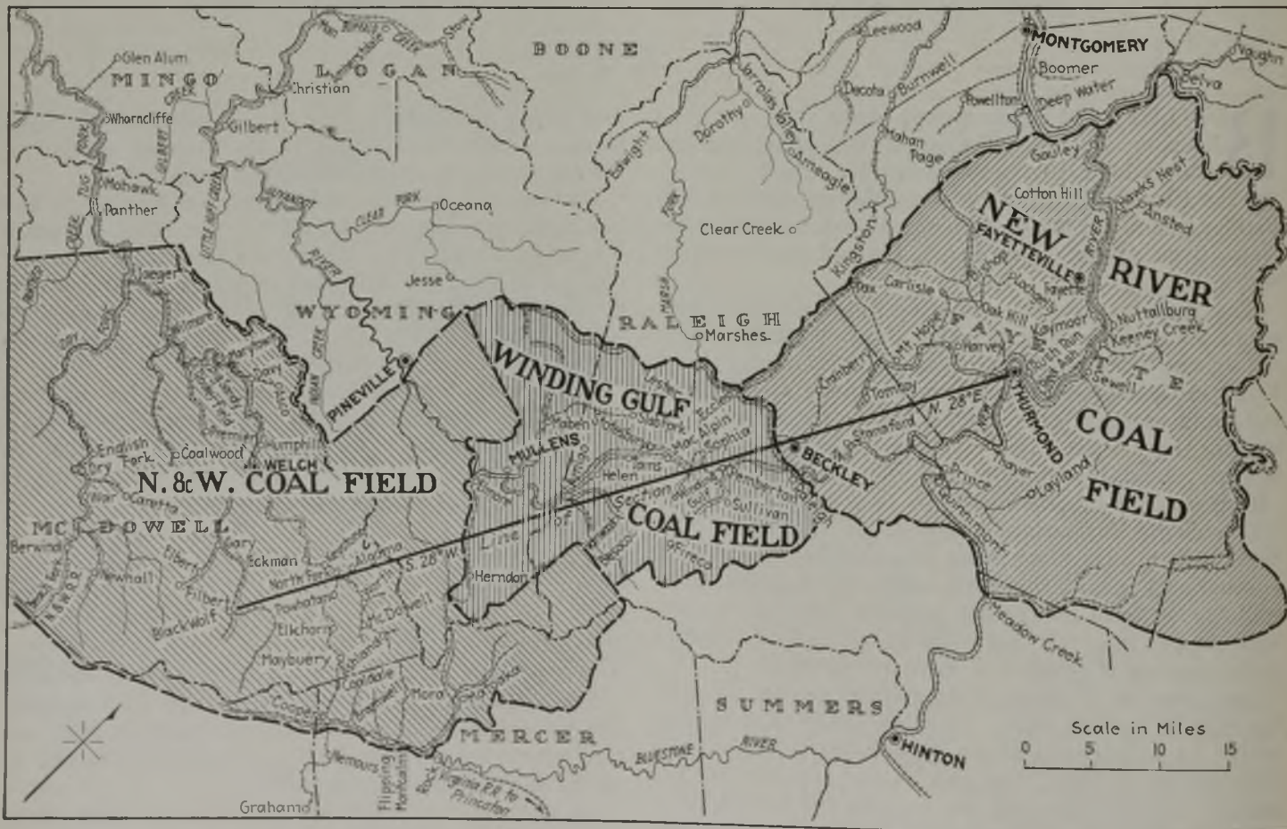
Fig. 1—Map of the Region Where Beckley Coal Is Found The line extending from Thurmond to Black Wolf is the line upon which the cross-section shown in Fig. 2 is taken
