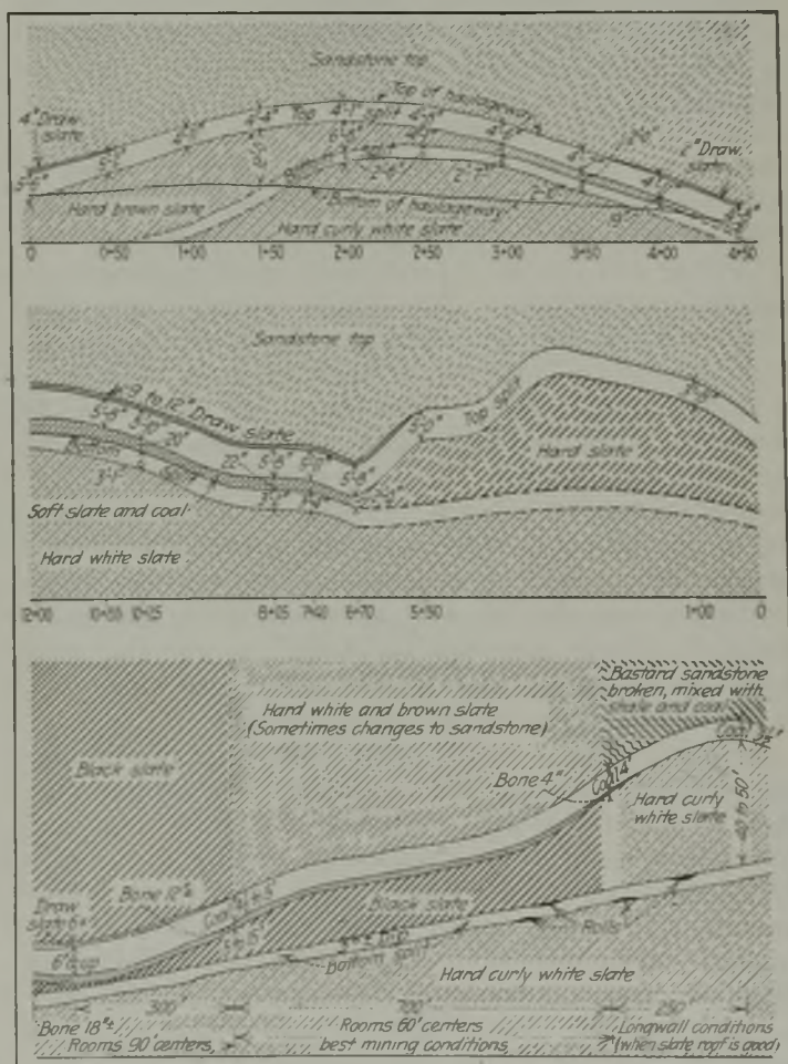
Fig. 3—Typical Cross-Sections of the Beckley Bed
