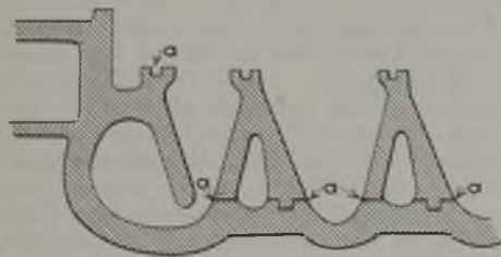
Fig. 1—Original Joint Between Separator and Casing
