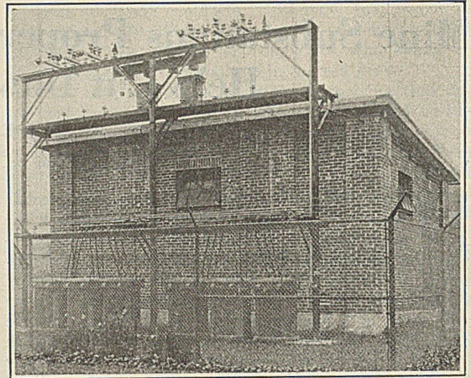
Permanent Substation Houses Two 150-Kw. Rotary Converters
