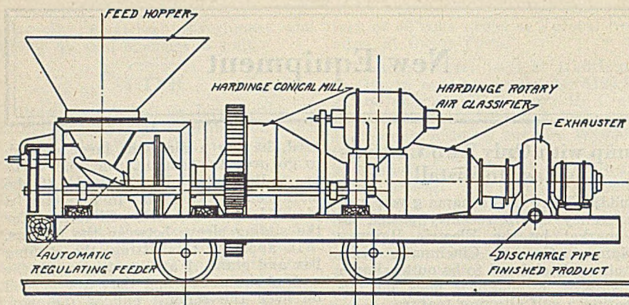
Arrangement of One-Car Pulverizing Unit
