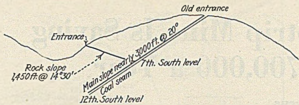
Fig. 3—Sketch of Surface Contour
