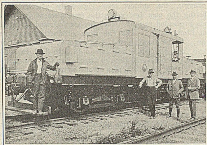
Sixty-Ton Storage Battery Locomotive
