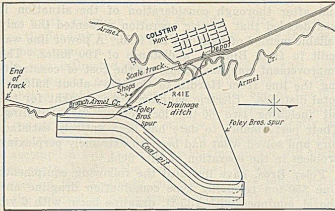
Fig. 1—Layout at Colstrip
