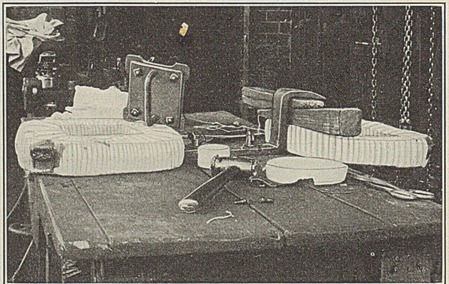
Test Gage and Bench Clamp Aid Repairman
