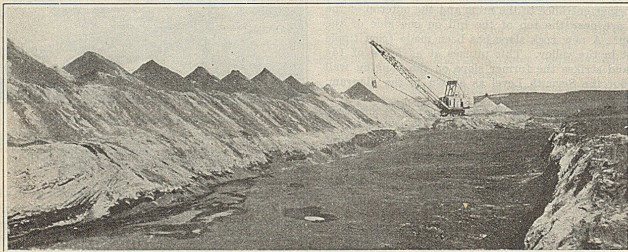
Through Cut at Colstrip Made by Big Shovel Working Part Time as Dragline
