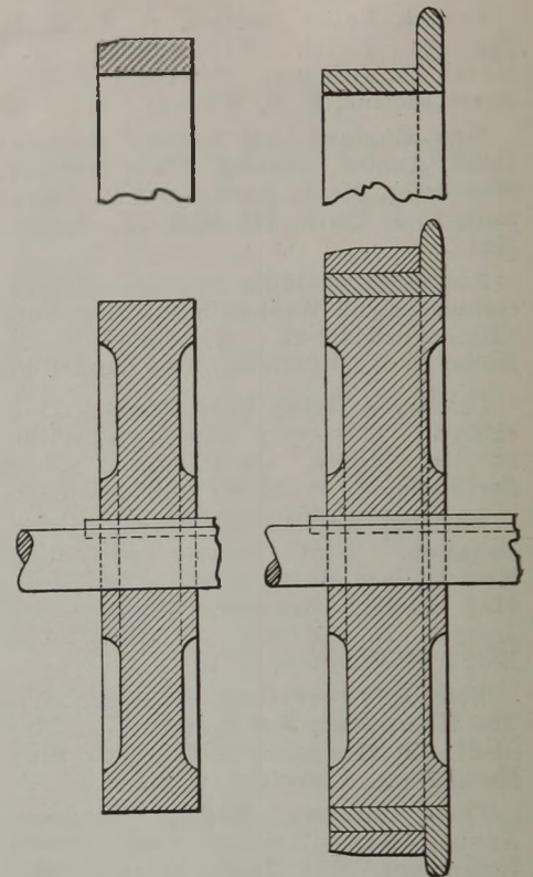
Cross-Sections of Wheel and Tire
