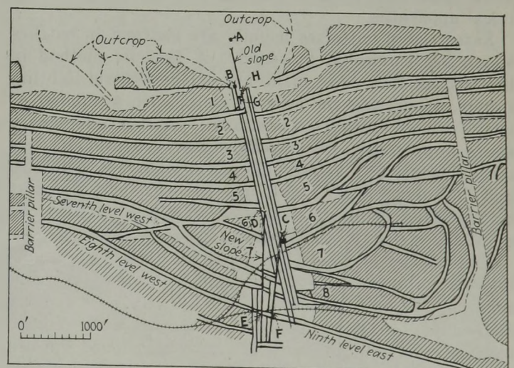
Slope in Roof Rock Decreases Maintenance Cost, Shortens Haul and Lowers Hoisting Lift
