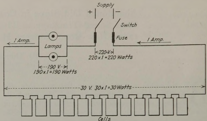
Fig. 1—Simple Charging Arrangement
