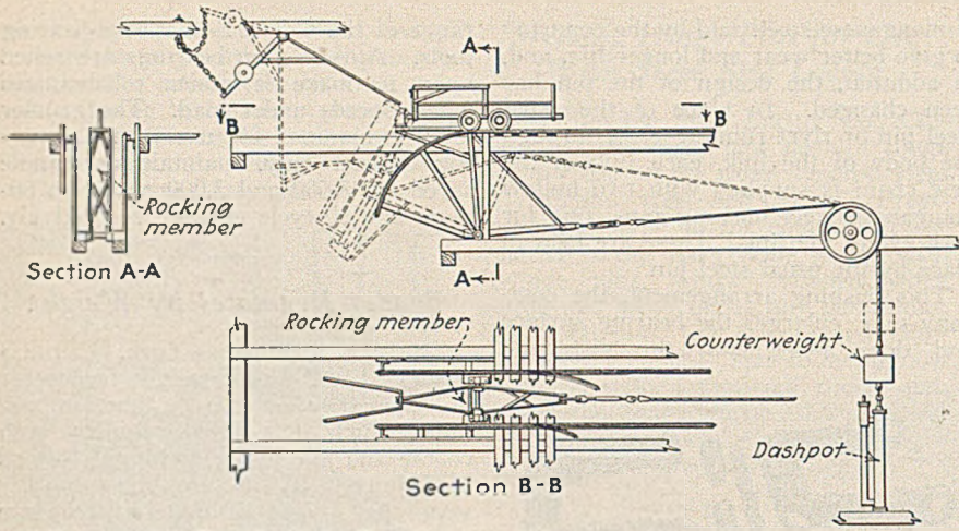
Construction Details of the Dump
