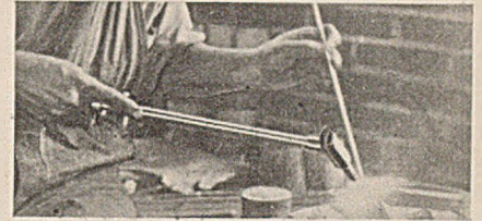
Welding Drill-Iron Shoulder
