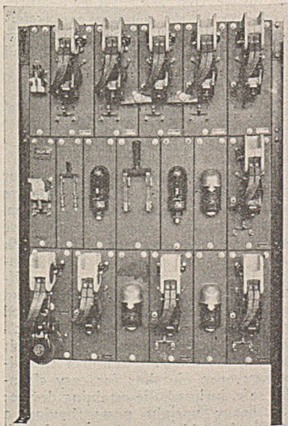
"Wright" Dynamic Lowering Circuit Controller
