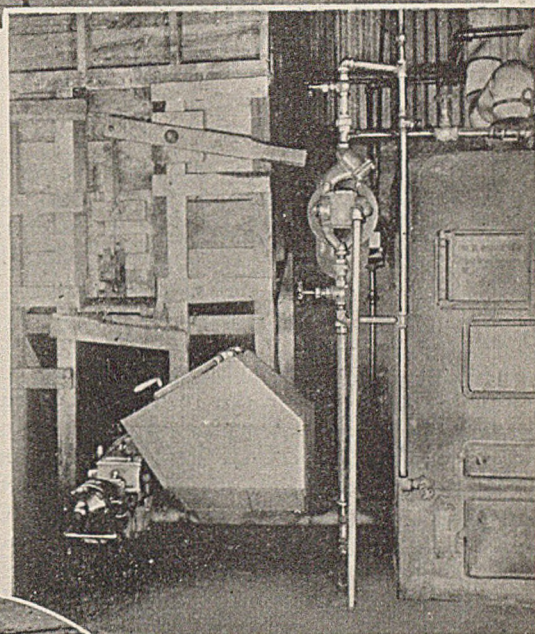
At the Gay Residence Even Loading of the Hopper Has Been Mechanized; Note the Lower Gate
