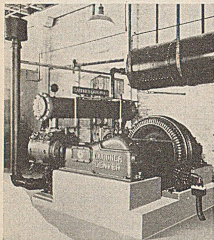
Synchronous Motor Driven Air Compressor
