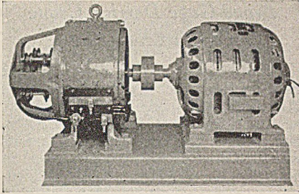
Motor-Generator Set With Welded Steel Base
