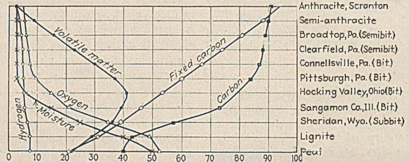
Fig. 2—Shows How Analytic Constituents Vary for a Selected Series of Coals—Superanthracite Omitted
