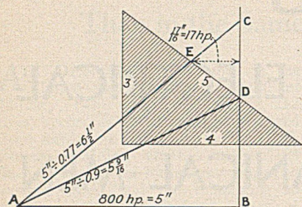
Determines Size of Synchronous Motor
