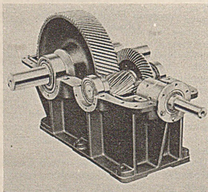
Falk Right Angle Drive-Speed Reducer
