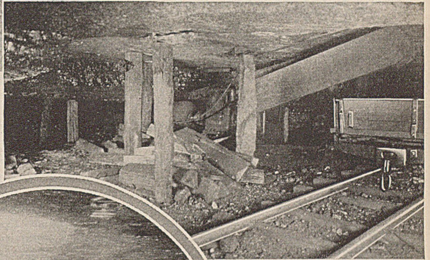
Fig. 3—Conveyor Set-Up at the Room Neck. Here Can Be Seen the 14 In. of Coal Above the Drawslate. At This Point the Latter Is Much Thinner Than Average
