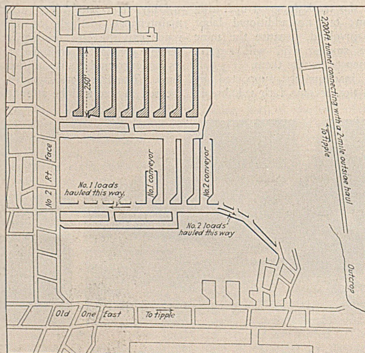
Fig. 1—Heavy Lines Indicate Area of "Old One East," Section Developed and Mined With Chain-Flight Conveyors
