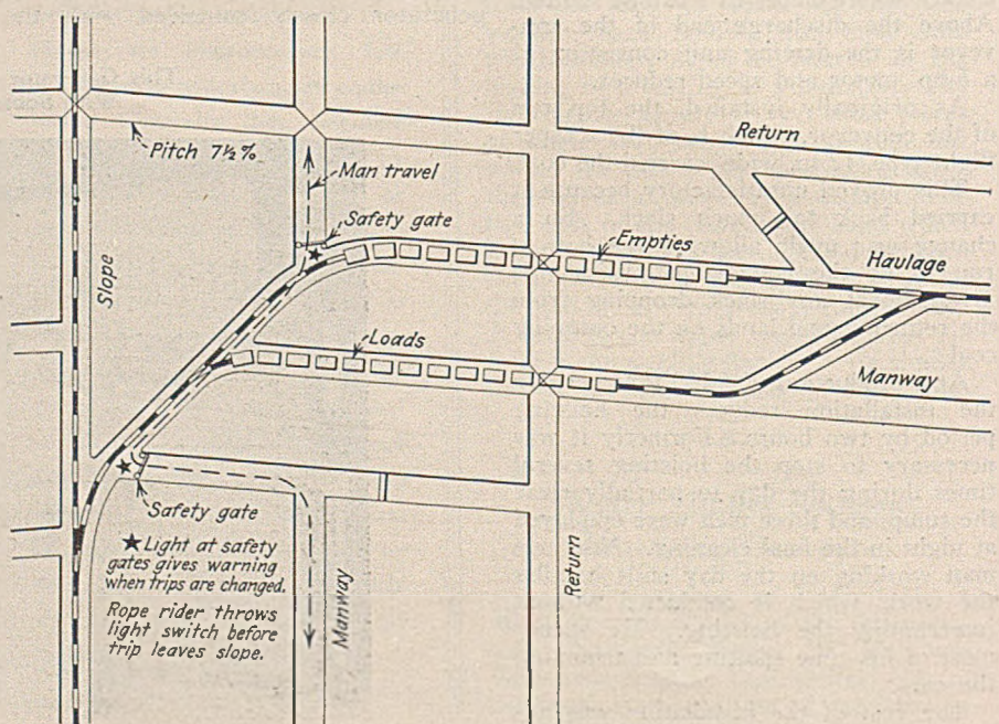
Parting and Manway Layout
