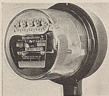
Westinghouse Detachable Watthour Meter
