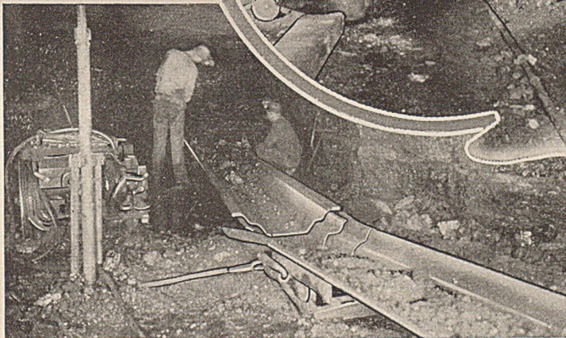
Fig. 5—One Man at the Control of the Duckbill and the Other Moving It Over With a Bar. Back of the Conveyor Pivot Jack at the Left Is a Shortwall Mining Machine
