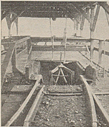
Showing Rocking Member in Position to Receive Loaded Car
