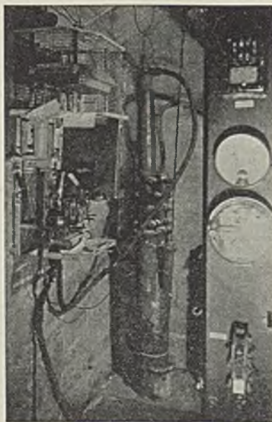
Top of borehole in surface substation at No. 4 mine, showing method of suspending the cables. At the left is the automatic reclosing breaker, installation of which is standard practice in all Superior substations.
