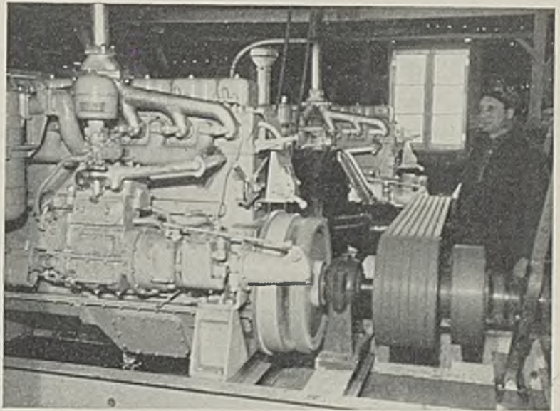
Two 125-hp. tractor-type diesels driving one 150-kw. generator replaced an antiquated steam plant. C. B. Aston, mine owner, stands at the right.
