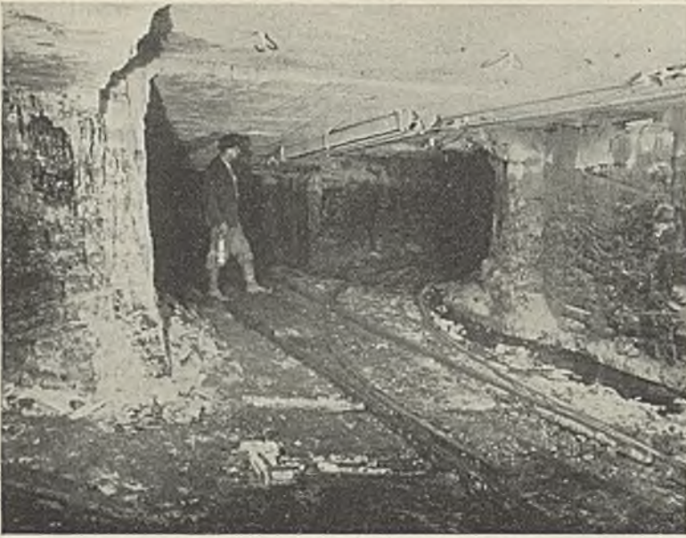
Butt heading in the machine section, Mona mine, showing parallel throw on the switch, guardboards on the trolley wire over a turnout into the parallel heading and rock dust on the ribs, top and floor. All places with track are rock-dusted every week end.
