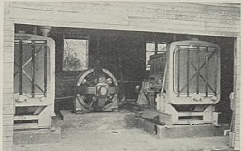
Engines are complete units with gasoline-engine starters and fan-cooled radiators.
