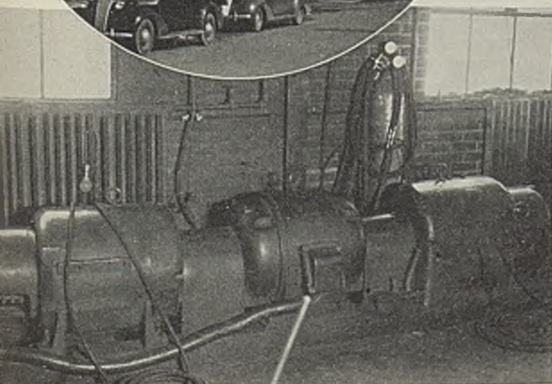
This dual welding unit was purchased for the new welding shop. Each generator is rated 300 amp.
