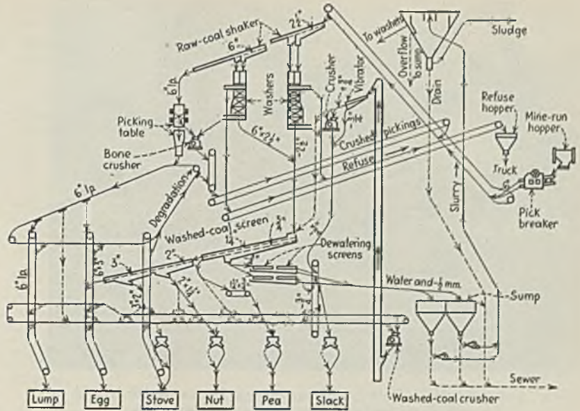
Fig. 1—Flow diagram, Sentry preparation plant
