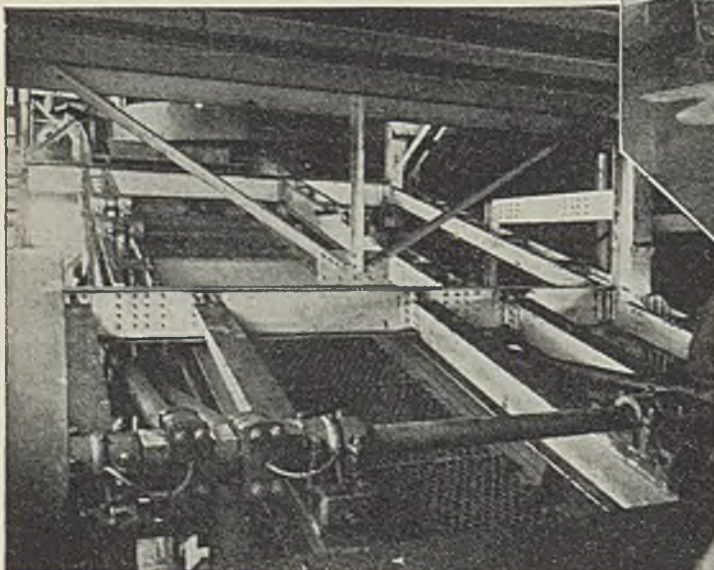
Six-inch lump is cleaned on this two-section shaking picking table. At the right are the reject elevators of the 6x2½-in. washer.
