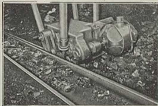
Shaking Conveyor Drives and Accessories in various Types and capacities for any mining requirement. Standard, explosion-proof and Government Approved permissible motors can be supplied for various current characteristics.
