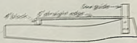
Fig. 1—Sawing method of securing uniform cuts for pitch of legs
