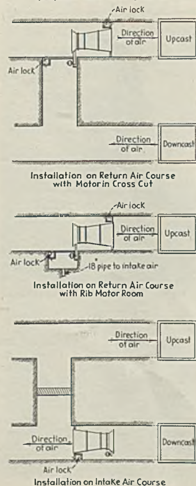
Fig. 1—Alternative methods of installing propeller fans underground.
