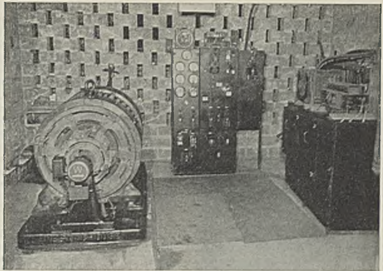
150-kw. full-automatic substation in No. 3 mine. By leaving openings in the blocks making up the front or back walls, or both, unauthorized entrance to station is prevented while air circulation is facilitated.
