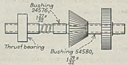
Diagrammatic sketch showing points where split bushings were installed
