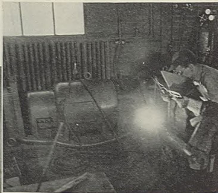
Building up a worn locomotive axle using coated electrode and current supplied by a new dual-unit machine standing in the background
