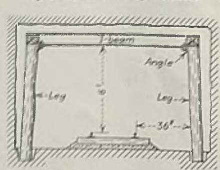
Fig. 3—Typical I-beam set, showing placement of angles to counteract side pressure
