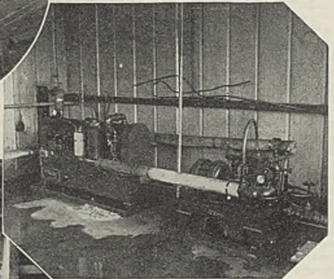
One of the two heating units used in heating the coal-treating fluid prior to application at Sentry.
