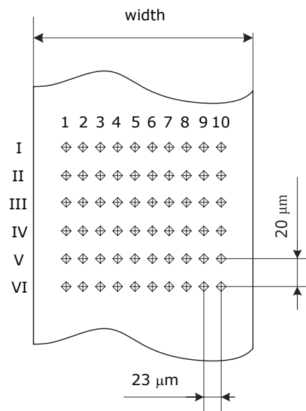
Fig. 1. The pattern of microhardness measurements
