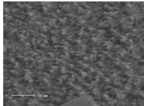
Fig. 18 a) Topography of the \text{TiN}+\text{TiAlSiN}+\text{AlSiTiN} and b) \text{TiN}+\text{Al}_2\text{O}_3 coatings surface deposited onto the \text{Si}_3\text{N}_4 nitride ceramics substrate
