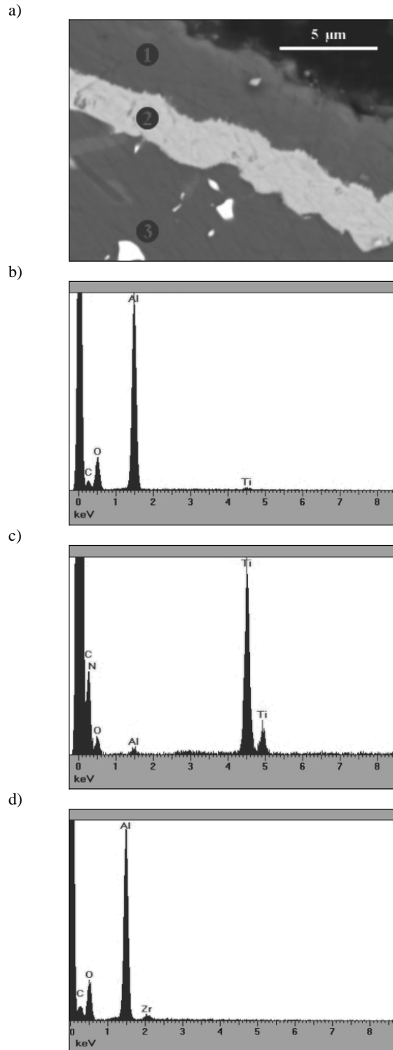
Fig. 14. a) Fracture surface of the TiN+Al 2 O 3 coating deposited on Al 2 O 3 +ZrO 2 substrate, b) X-ray energy dispersive plot the area 1 as in figure a, c) X-ray energy dispersive plot the area 2 as in figure a, d) X-ray energy dispersive plot the area 3 as in figure a.
