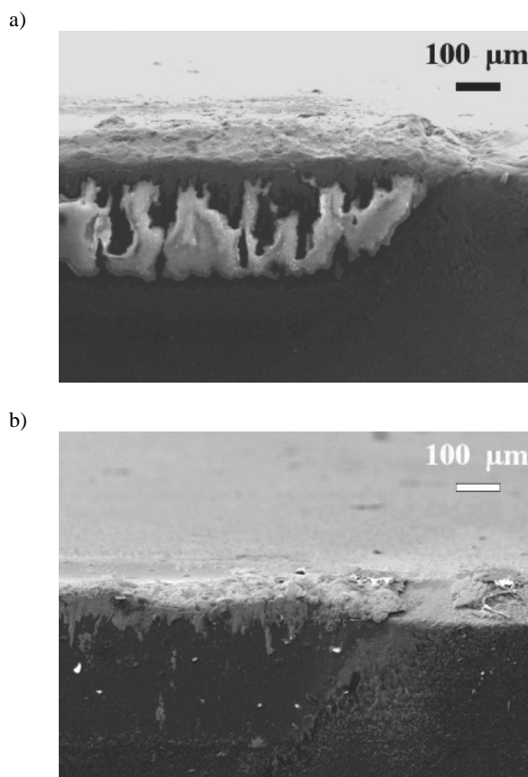
Fig. 30. Flank wear character of the: a) \text{Al}_2\text{O}_3+\text{ZrO}_2 ceramics with \text{TiN}+\text{multi}(\text{Ti},\text{Al},\text{Si})\text{N}+\text{TiN} , b) uncoated \text{Al}_2\text{O}_3+\text{ZrO}_2 ceramics during the continuous cutting of the EN-GJL-250 grey cast iron
