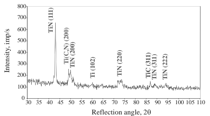
Fig. 19. X-ray diffractions pattern of the cermets with the \text{TiN}+(\text{Ti,Al,Si})\text{N}+\text{TiN} gradient coating
