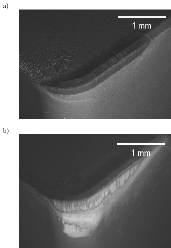
Fig. 29. Width of the VB tool flank for: a) nitride ceramics \text{Si}_3\text{N}_4 with deposited \text{TiN}+\text{Al}_2\text{O}_3 coating, b) uncoated \text{Si}_3\text{N}_4 nitride ceramics – after 8 minutes of machining
