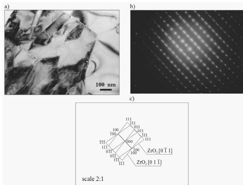
Fig. 3. Structure of \text{Al}_2\text{O}_3+\text{ZrO}_2 substrate: thin foil structure parallel to the layer surface (TEM): a) bright field, b) diffraction pattern from the area as in figure a, c) solution of the diffraction patterns from figure b (2:1 scale)
