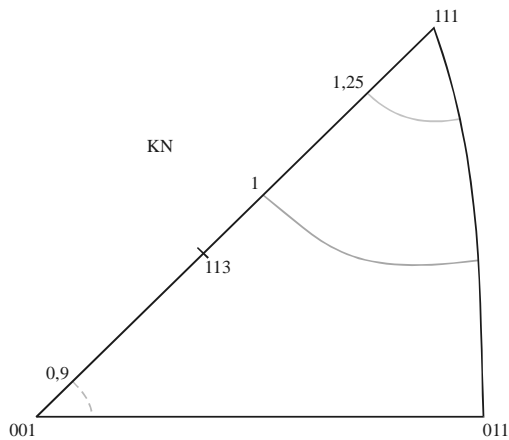
Fig. 22. Exemplary inverse for \text{TiN} layer representing the distribution of normal to the \text{TiN} + \text{multiTiAlSiN} + \text{TiN} coating surface in the (001)-(011)-(111) base triangle (KN - normal direction)
