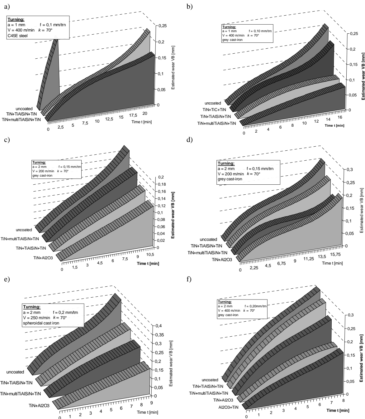
Fig. 32. Comparison of the functional properties of investigated materials: a) cemented carbides, b) cermets, c) \text{Al}_2\text{O}_3+\text{ZrO}_2 , d) \text{Al}_2\text{O}_3+\text{TiC} , e) \text{Al}_2\text{O}_3+\text{SiC}_{(w)} and f) \text{Si}_3\text{N}_4 nitride ceramics
