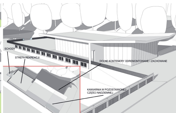
Rys. 5. Szkic wariantu 4 Fig. 5. Scetch of variant 4
