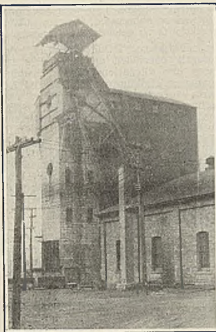
Concrete Headframe at Brier Hill
