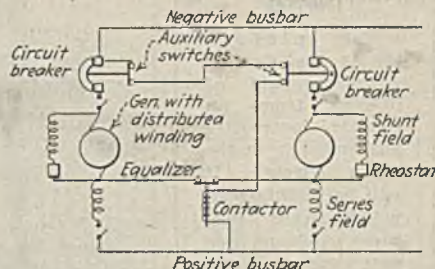
Fig. 2—Equalizer Switch Cures Flashes But Auxiliary Switches Fail
